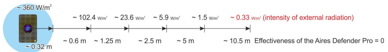
Fig. 1. Scale of the drop in the effectiveness of protection from the Aires Defender Pro.
