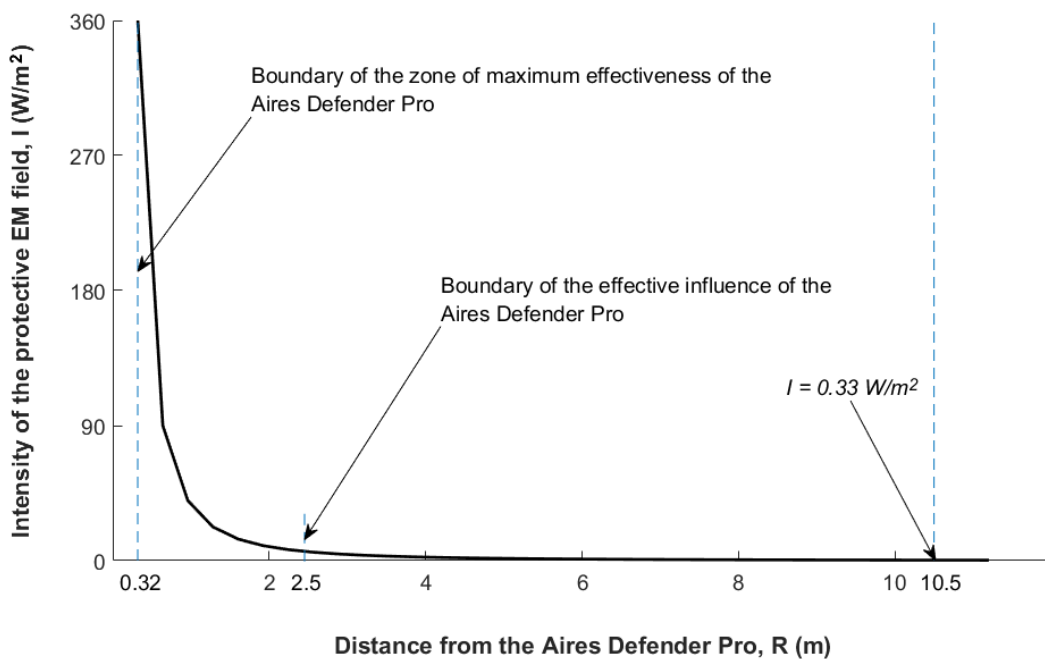
Fig. 2. Graph of the effectiveness of the Aires Defender Pro as a function of distance.
